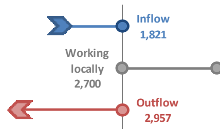
Estimated Worker Commuting Flows To and From Lyon County
