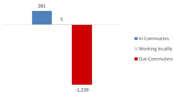
Figure 18. Commuting Inflows and Outflows: Fairfax
